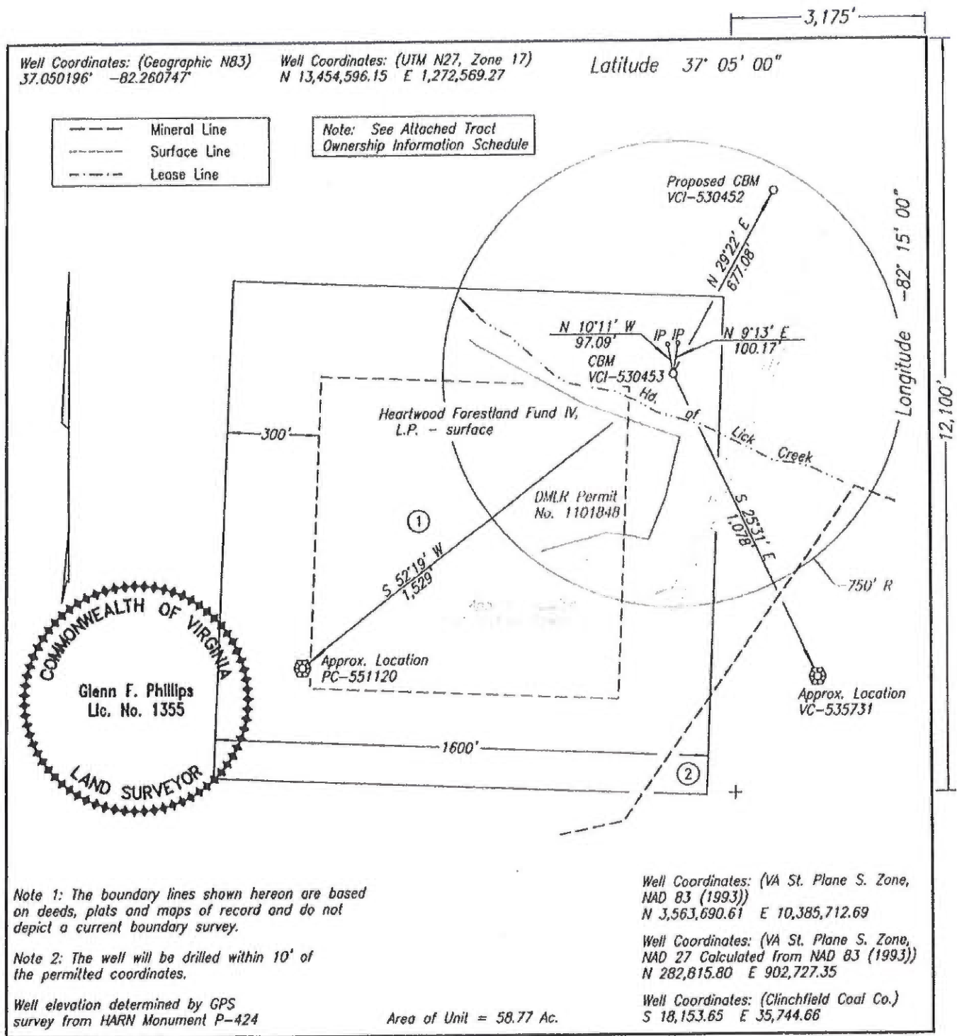
WELL LOCATION PLAT NORA GRID BM-59
