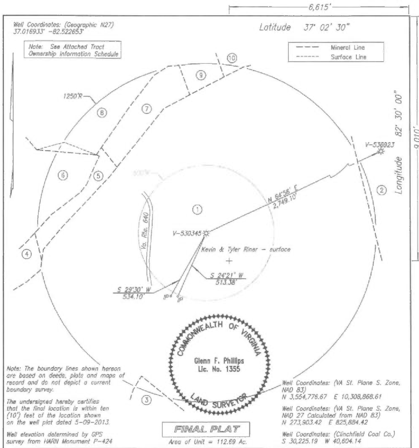
WELL LOCATION PLAT NORA GRID BT-12
