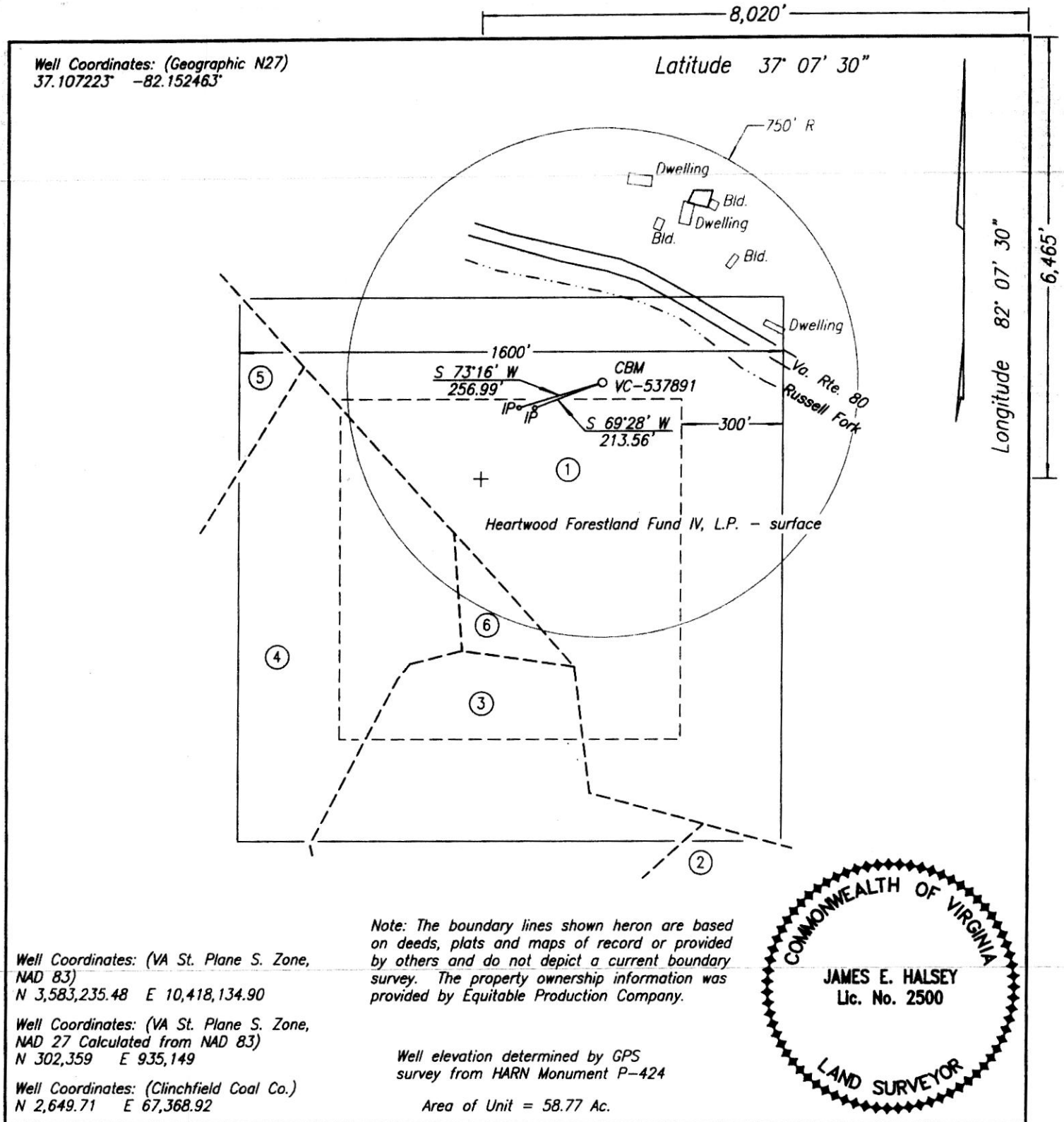
WELL LOCATION PLAT (Nora Grid AZ-79)
