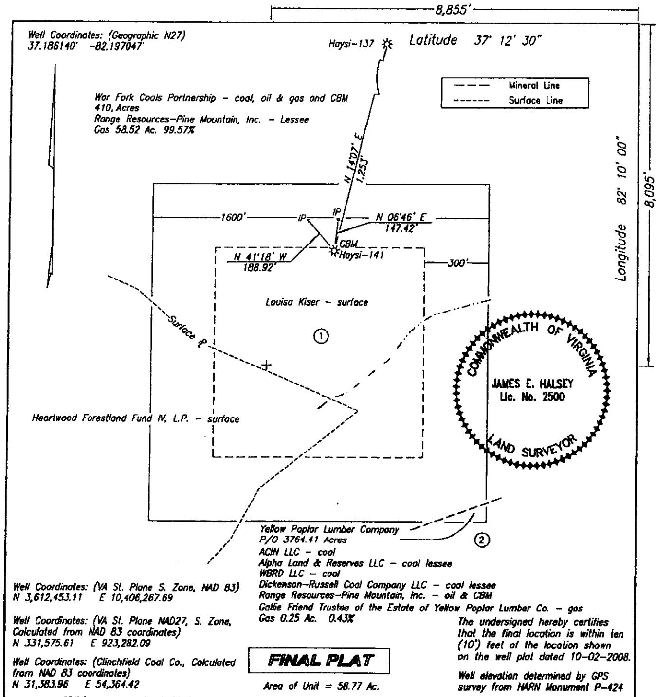
WELL LOCATION PLAT (Nora Grid AH-71)
